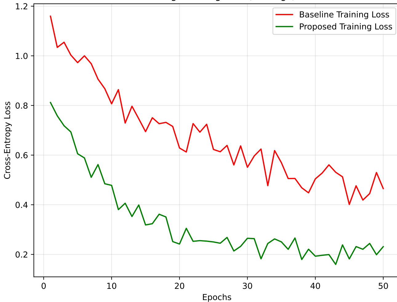
Training Convergence (50 Bags)
